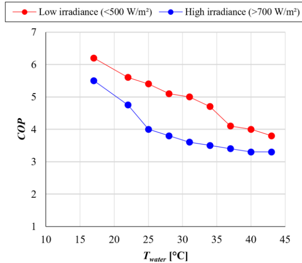
Figure 3: COP Analysis of the SAHP System
