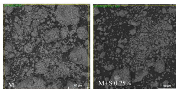
Figure 12. Morphology and topography of type N cement mixtures with Crab Nanoparticles.
