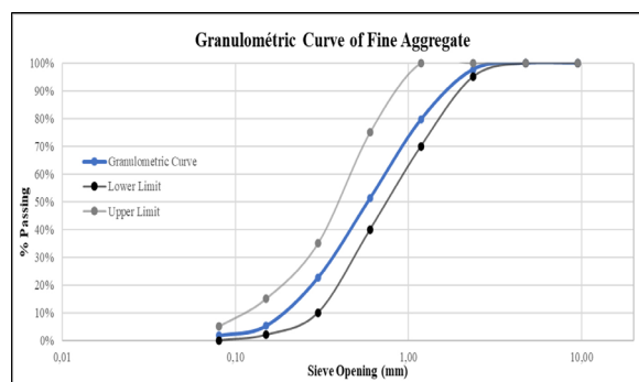
Figure 3. Granulometric of aggregate
