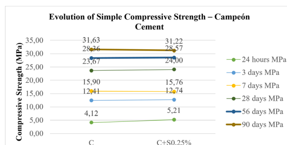
Figure 9. Evolution of Compressive Strength – “Campeón” Cement
