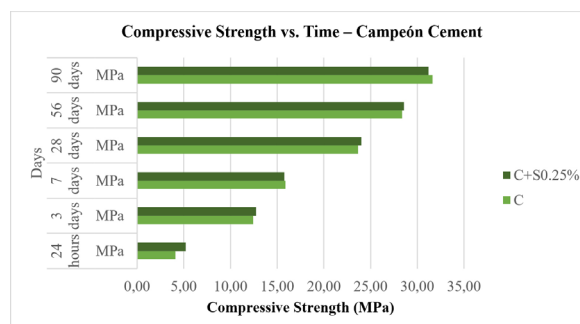
Figure 8. Compressive Strength vs Time – “Campeón” Cement
