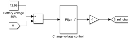
Figure 5: Discrete PI control for charge voltage control
