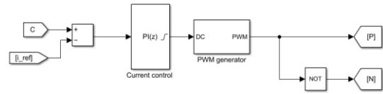
Figure 4: Discrete PI control for control of IGBTs
