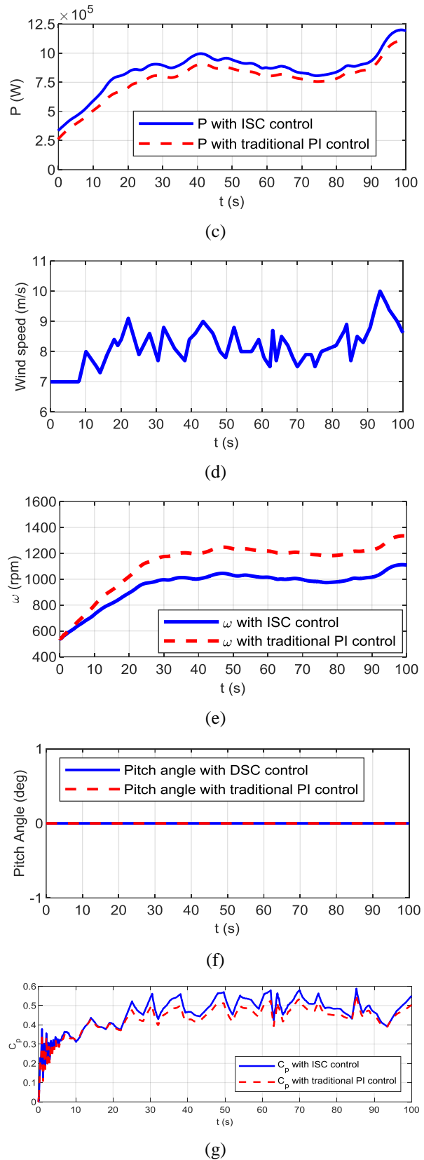
Figure 12: Steady wind speed with realistic inputs: Reference signal i_{qr} in p.u. (a), electromagnetic torque in Nm (b), active output power in W (c), wind input in m/s (d), generator speed in rpm (e), pitch angle in degrees (f) and C_p (g)
