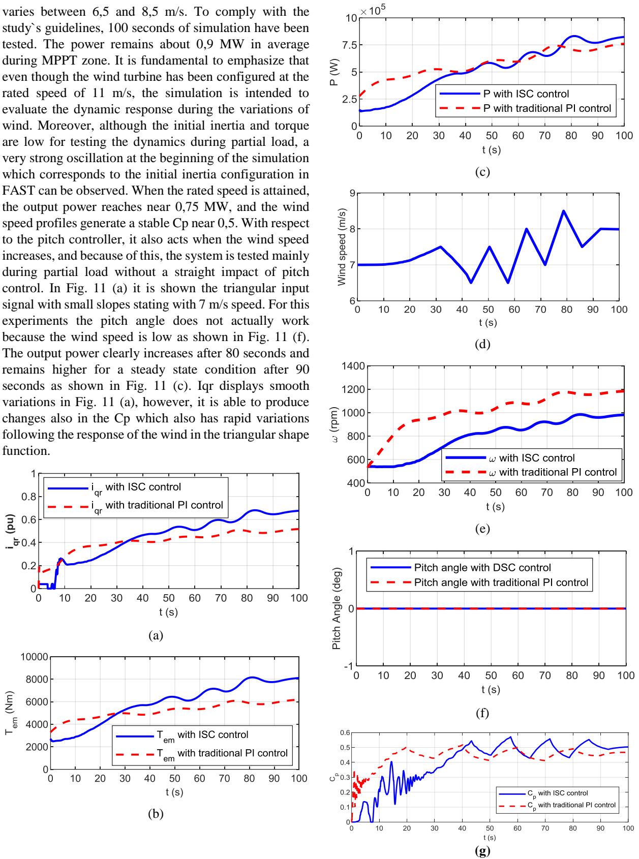
Figure 11: Steady wind speed with positive and negative ramp: Reference signal i_{qr} in p.u. (a), electromagnetic torque in Nm (b), active output power in W (c), wind input in m/s (d), generator speed in rpm (e), pitch angle in degrees (f) and C_p (g)
